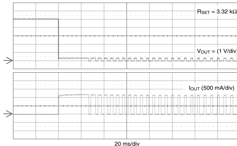
Figure 2. Current Over load Condition. Load Switch turned on with 0.1 \Omega load at time = 0 ms.
