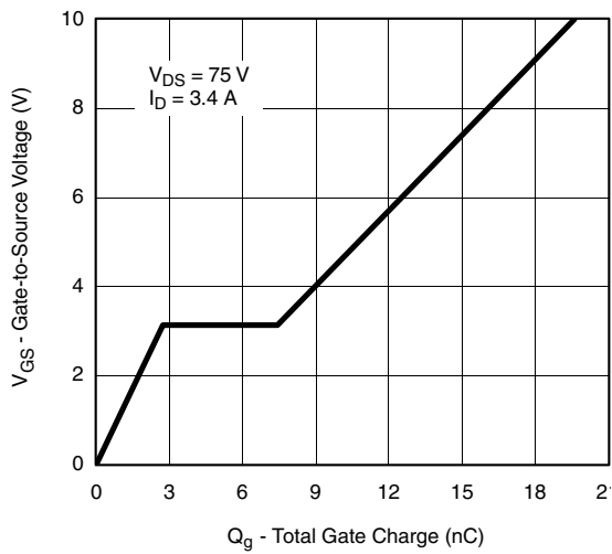
Gate Charge
