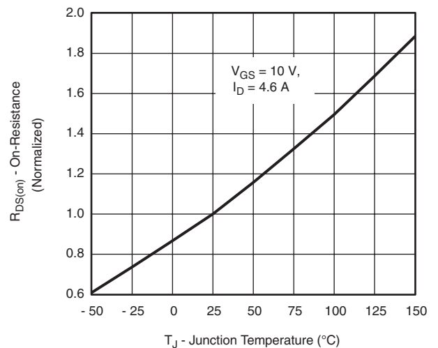
V_{GS} = 10\text{ V} , I_D = 4.6\text{ A} T_J - Junction Temperature ( ^\circ\text{C} ) On-Resistance vs. Junction Temperature
