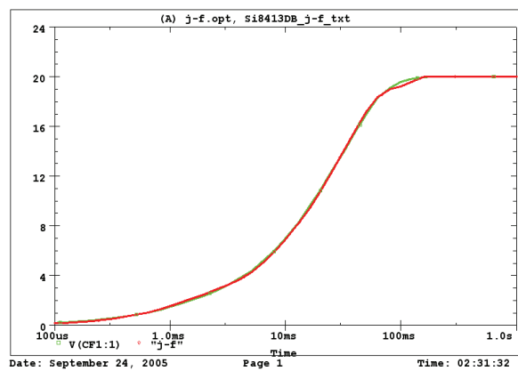
Si8413DB Filter j-f Temperature: 27.0
