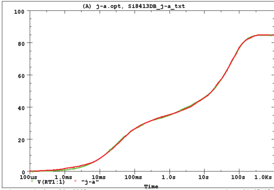
Si8413DB Tank j-a Temperature: 27.0
