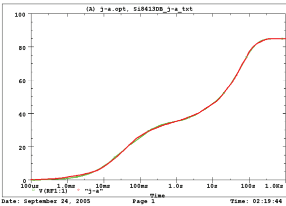
Si8413DB Filter j-a Temperature: 27.0
