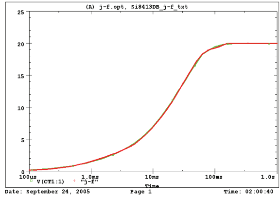
Si8413DB Tank j-f Temperature: 27.0
