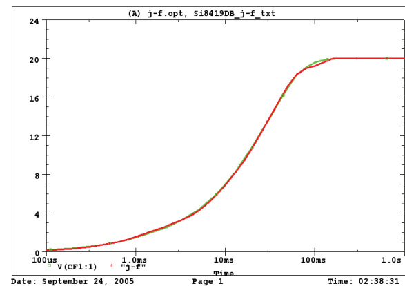
Si8419DB Filter j-f Temperature: 27.0
