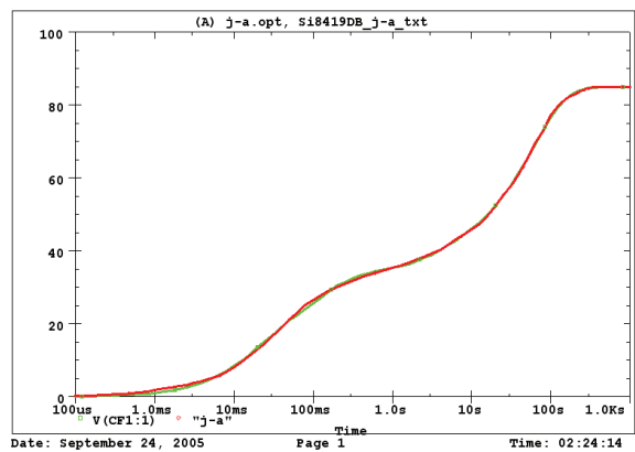
Si8419DB Filter j-a Temperature: 27.0
