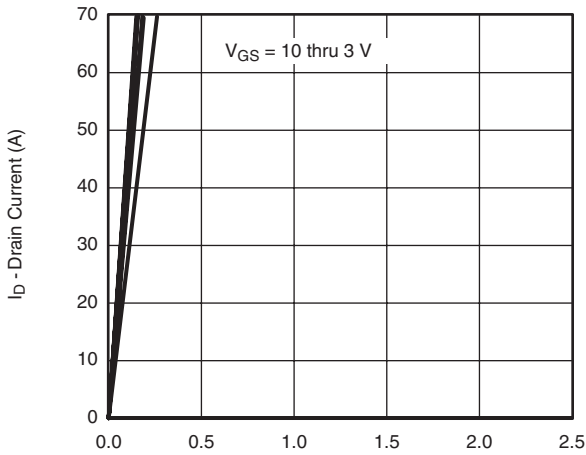
V_{GS} = 10 thru 3 V Output Characteristics
