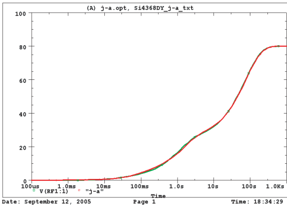
Si4368DY Filter j-a Temperature: 27.0
