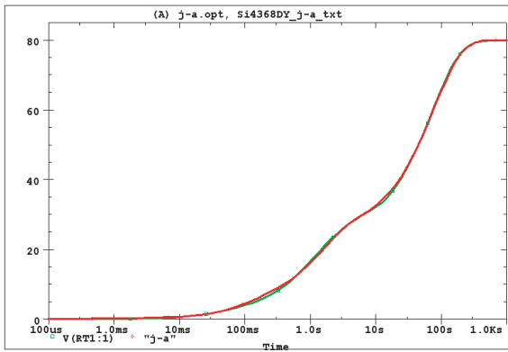
Si4368DY Tank j-a Temperature: 27.0
