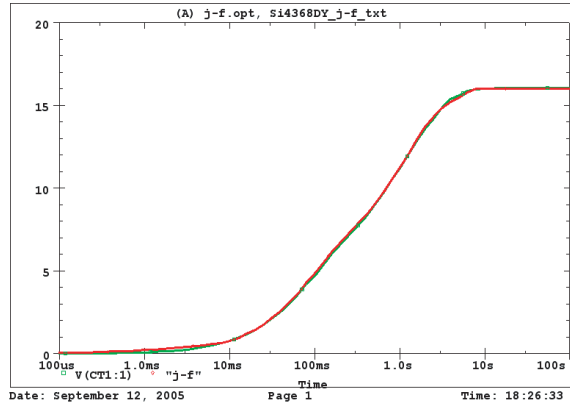
Si4368DY Tank j-f Temperature: 27.0
