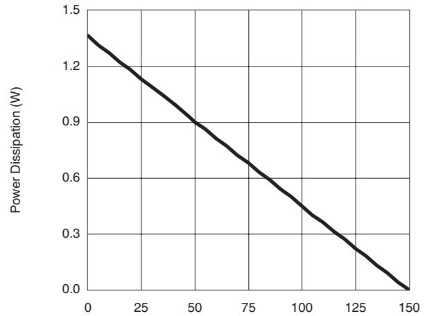
T_A – Ambient Temperature (°C) Power Derating, Junction-to-Ambient
