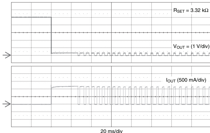
Figure 2. Current Over load Condition. Load Switch turned on with 0.1 \Omega load at time = 0 ms.
