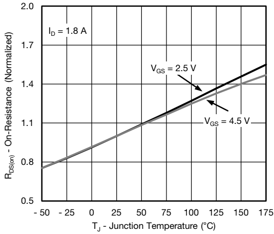
On-Resistance vs. Junction Temperature (1.8 V)
