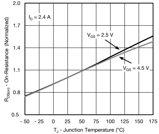
On-Resistance vs. Junction Temperature (2.4 V)
