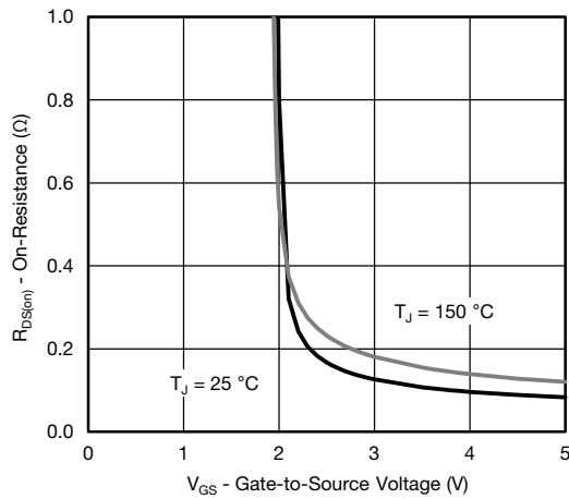
On-Resistance vs. Gate-to-Source Voltage (1.8 V)
