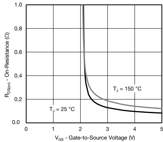
On-Resistance vs. Gate-to-Source Voltage (2.4 V)
