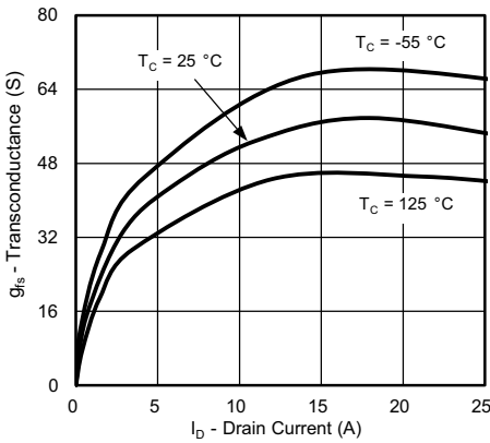
Transconductance
