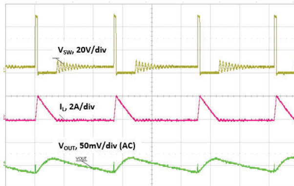
Fig. 33 - Output Ripple 300 mA, Time = 5 \mu s/div
