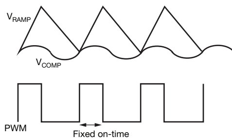
Fig. 6 - Operational Principle
