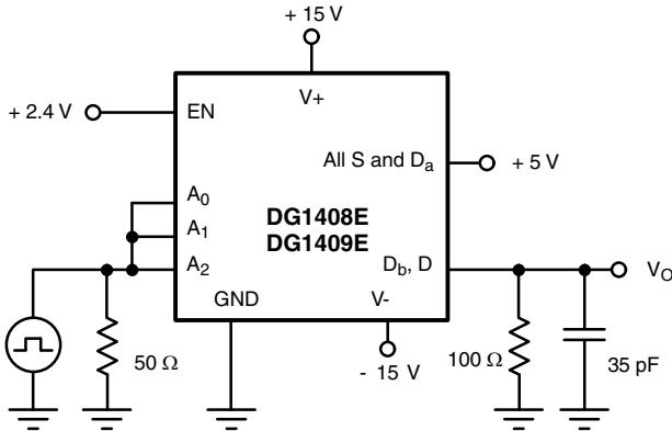
Fig. 3 - Break-Before-Make Internal
