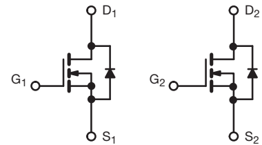
N-Channel MOSFET
