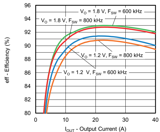
Fig. 1 - Efficiency vs. Output Current (V_{IN} = 12\text{ V}, L = 150\text{ nH}, V_{CC} = V_{DRV} = 5\text{ V})
