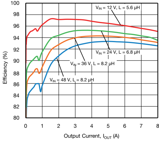
Fig. 16 - SiC477 Efficiency vs. Output Current, VOUT = 5 V
