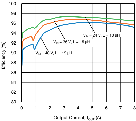
Fig. 17 - SiC477 Efficiency vs. Output Current, VOUT = 12 V
