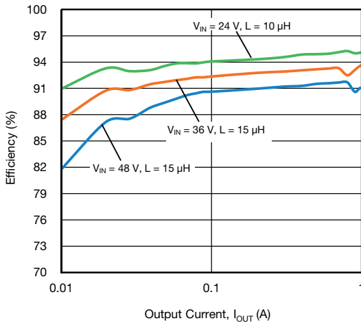
Fig. 20 - SiC477 Efficiency vs. Output Current - Light Load, VOUT = 12 V
