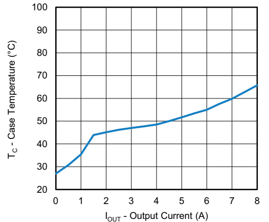
Fig. 21 - SiC477 Load Current vs. Case Temperature, VIN = 48 V, VOUT = 12 V
