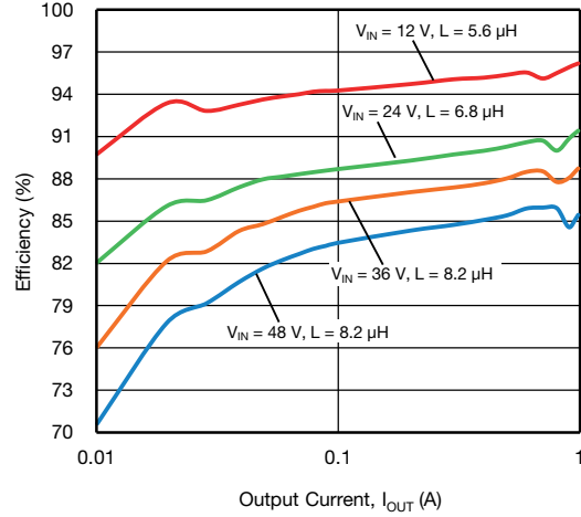
Fig. 19 - SiC477 Efficiency vs. Output Current - Light Load, VOUT = 5 V
