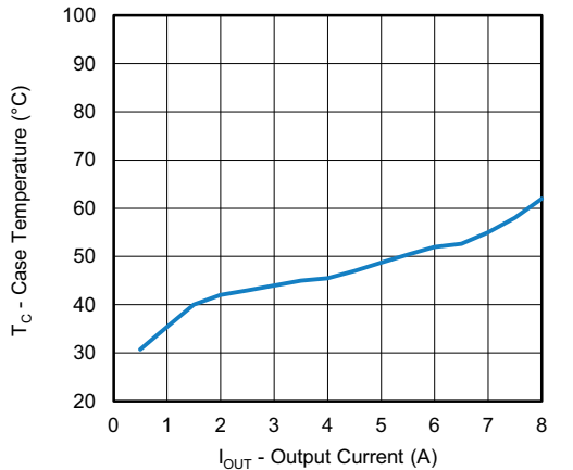
Fig. 18 - SiC477 Load Current vs. Case Temperature, VIN = 48 V, VOUT = 5 V
