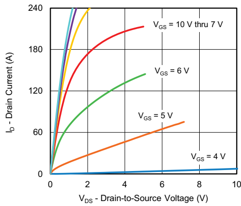
Output Characteristics
