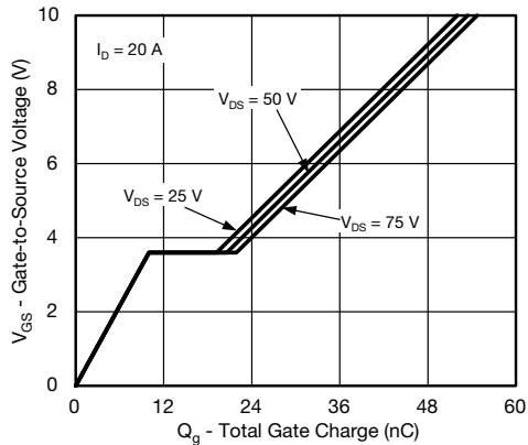
Gate Charge
