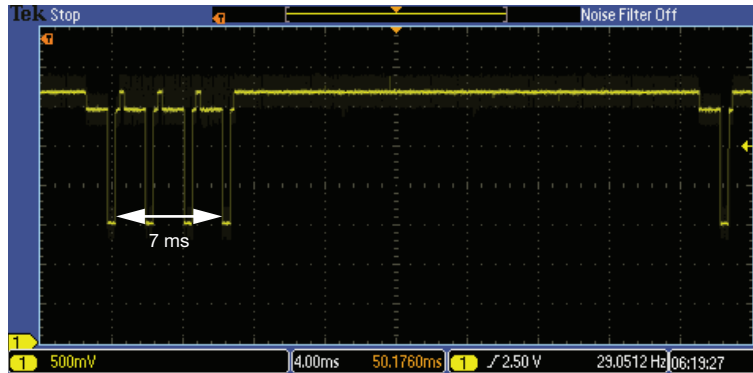
Fig. 32 - Smart Persist With PS_IT = 8T = 400 \mu s and PS_Period = 40 ms
