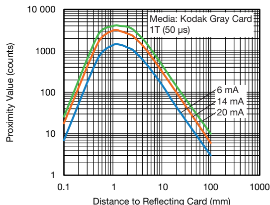
Fig. 12 - Proximity Value vs. Distance for 1T
