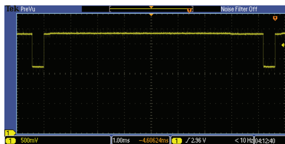
Fig. 14 - Proximity Measurements with PS_Period = 10 ms
