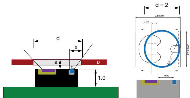
Fig. 9 - Window Dimensions for One Hole
