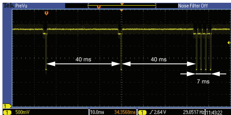
Fig. 33 - Always About 7 ms for These 4 Hits, Also When PS_Period is Programmed to Just 10 ms
