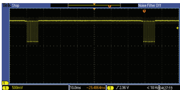
Fig. 37 - PS_Period = 80 ms and PS_IT = 8T (400 \mu s) and MPS = 8
