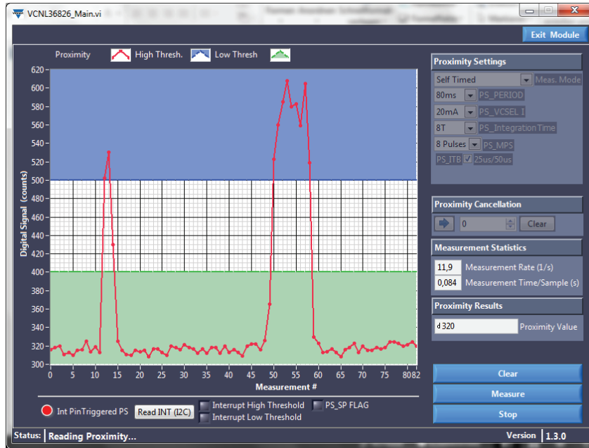
Fig. 27 - Hand in About 5 cm Distance for More Than 4 Consecutive Measurements Above Higher Threshold
