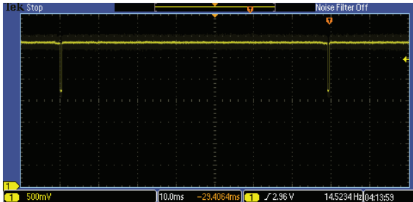
Fig. 15 - Proximity Measurements with PS_Period = 80 ms
