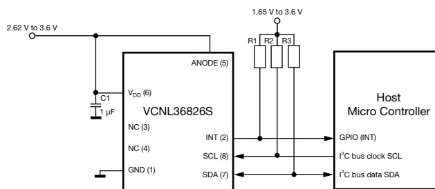
Fig. 5 - VCNL36826S Application Circuit
