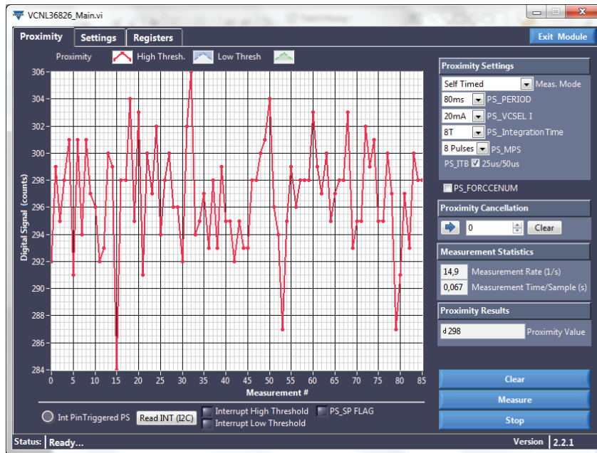
Fig. 23 - Screenshot of VCNL36826 Demo Software
