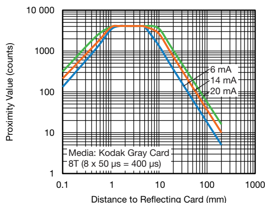
Fig. 13 - Proximity Value vs. Distance; PS_IT = 8T
