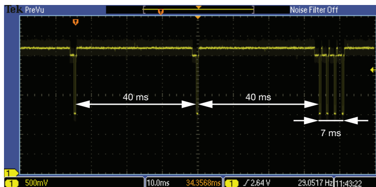
Fig. 34 - Smart Persist With Four Consecutive Proximity Pulses Short After Each Other
