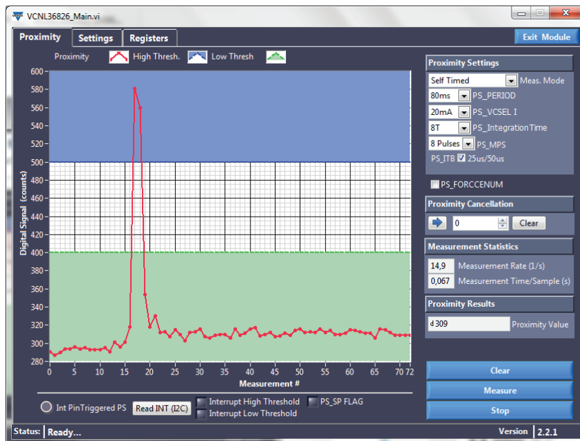
Fig. 26 - Upper and Lower Threshold Set and Hand in About 5 cm Distance
