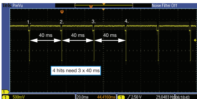
Fig. 31 - Interrupt Active After 4 Hits Above Threshold
