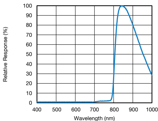
Fig. 10 - Spectral Sensitivity of the Proximity Photodiode
