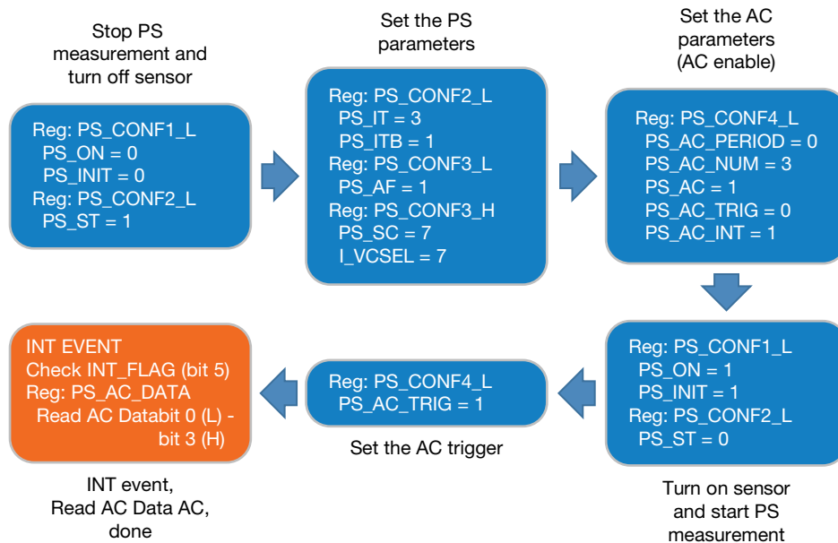
Fig. 39 - Software Flow Chart (for auto / dynamic calibration)
