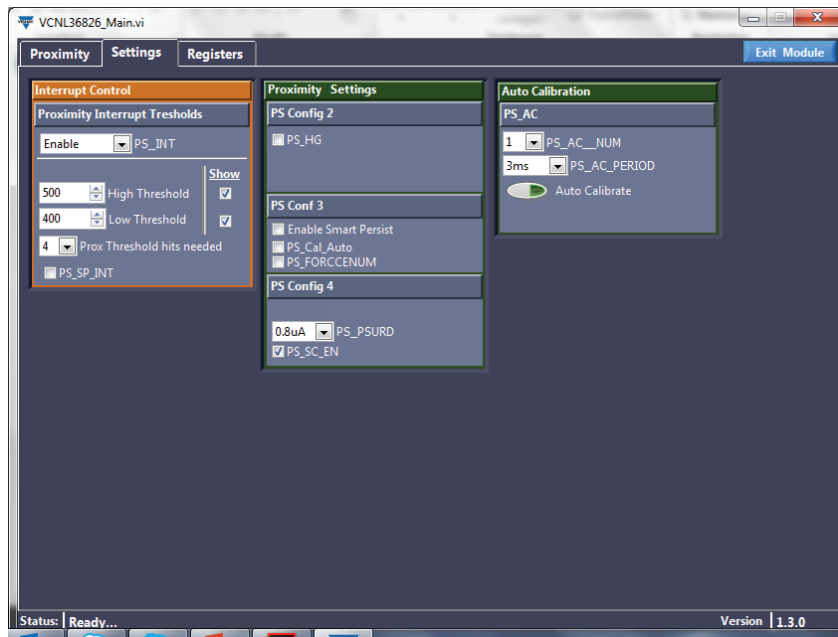
Fig. 25 - “Settings” Menu Within Demo Software
