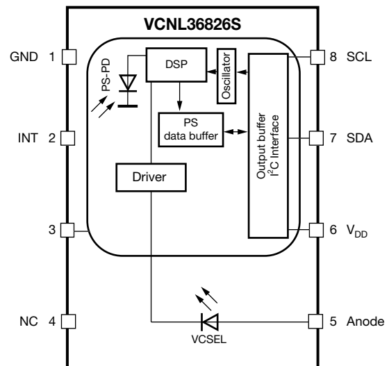
Fig. 3 - VCNL36826S Detailed Block Diagram
