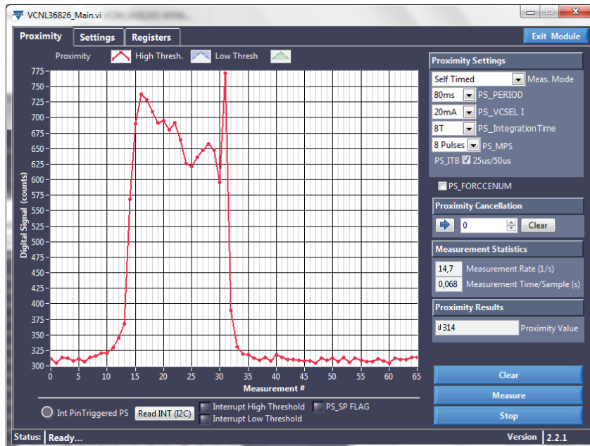
Fig. 24 - Hand in About 5 cm Distance Will Lead to More Than 500 Counts
