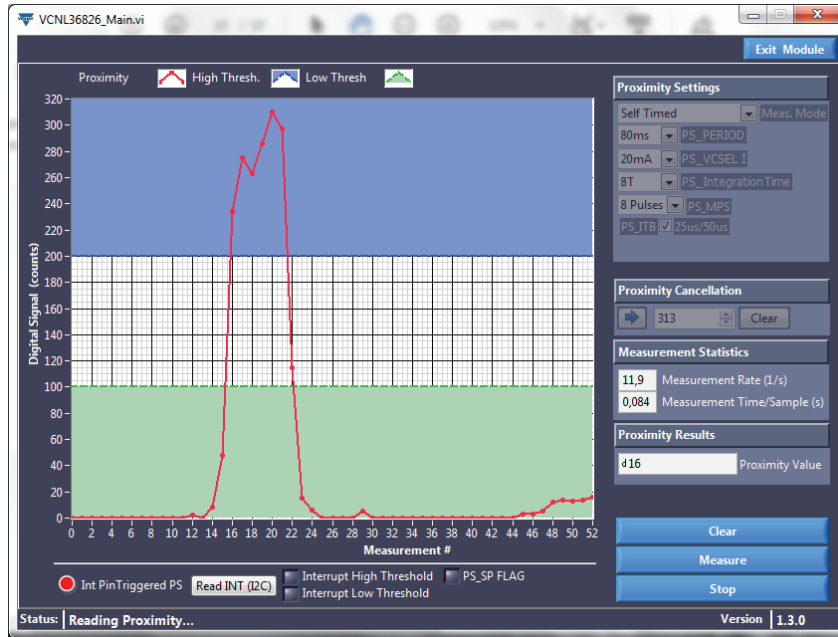
Fig. 29 - New Defined Thresholds With Cancellation Feature
