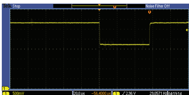
Fig. 11 - Proximity VCSEL Pulse for 1T
