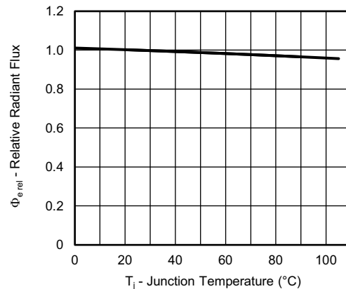
Fig. 6 - Relative Radiant Power vs. Junction Temperature
