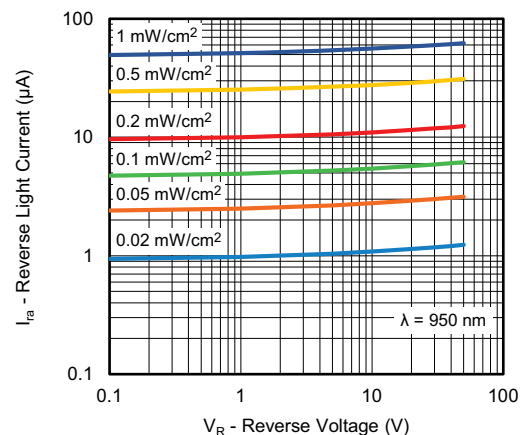
Fig. 4 - Reverse Light Current vs. Reverse Voltage
