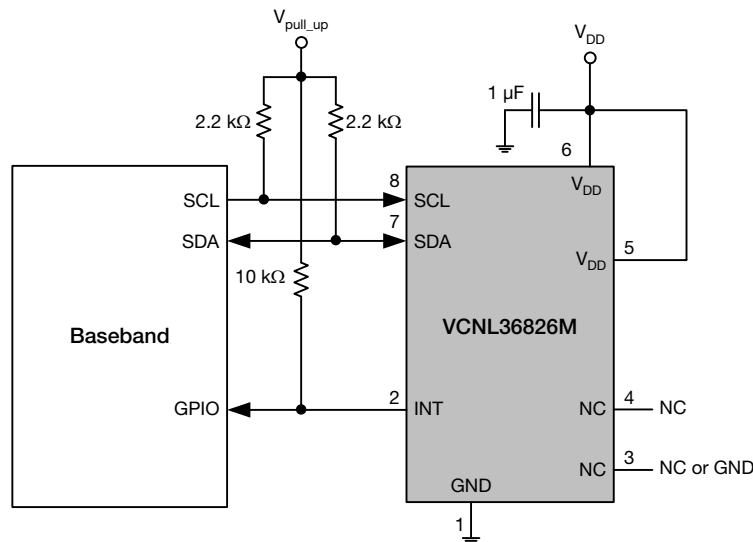
Fig. 11 - VCNL36826M Reference Circuit Connection With Host (proximity detection logic output mode) (VCNL36826M INT pin connecting to BB GPIO instead of INT pin)
