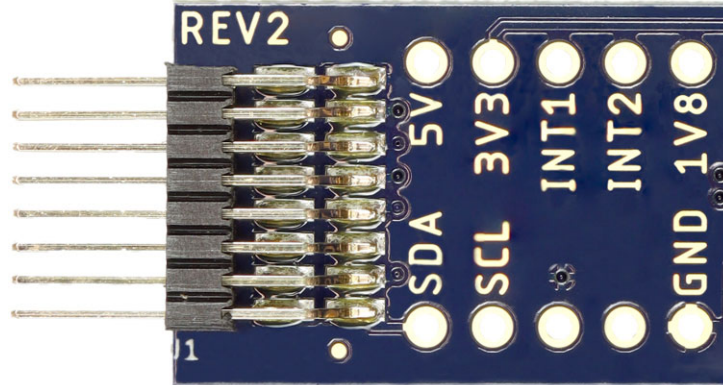
Fig. 3 - Connection of the Sensor Board (power supply and I 2 C lines)
