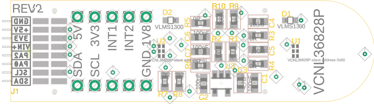
Assembly top
