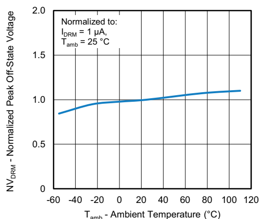
Fig. 6 - Normalized Peak Off-State Voltage vs. Ambient Temperature
