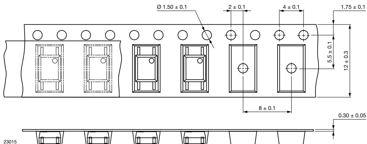
Fig. 10 - Tape and Reel Packaging (3000 pieces on reel)
