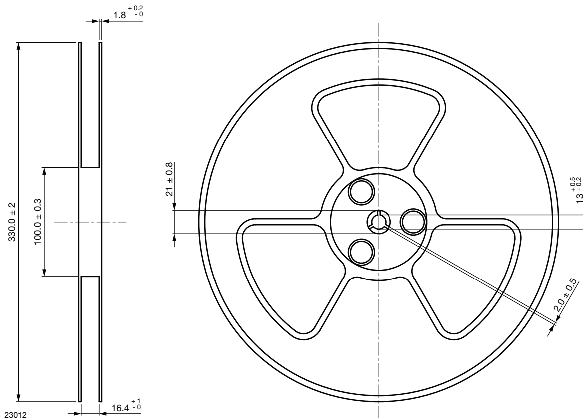
Fig. 11 - Tape and Reel Shipping Medium
