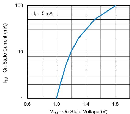
Fig. 4 - On State Current vs. On State Voltage
