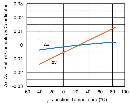
Fig. 11 - Shift of Chromaticity Coordinates vs. Junction Temperature
