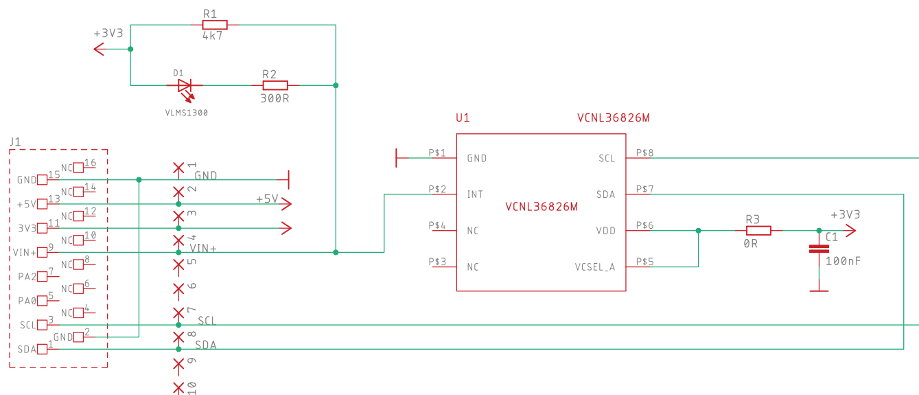
VCNL36826M sensor board, rev. 1.0
