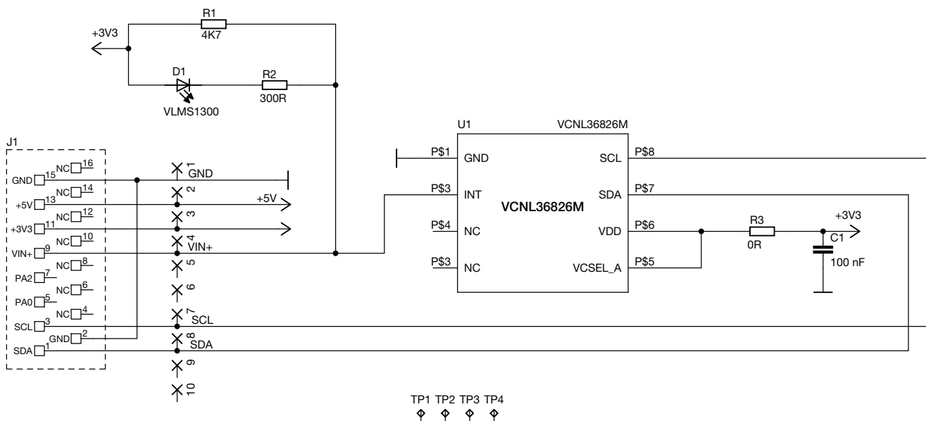
Fig. 7 - Schematic of the VCNL36826M Sensor Board
