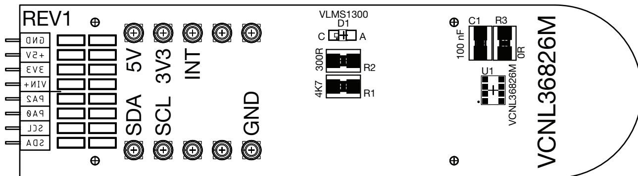
Assembly top
