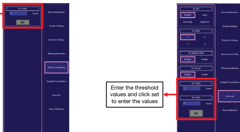
Fig. 5 - Offset Cancellation and Threshold Settings for the Interrupt
