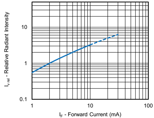
Fig. 5 - Relative Luminous Intensity vs. Forward Current
