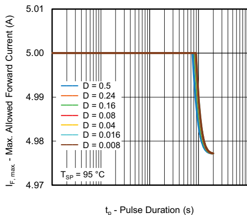
Fig. 9 - Max. Allowed Forward Current vs. Pulse Duration
