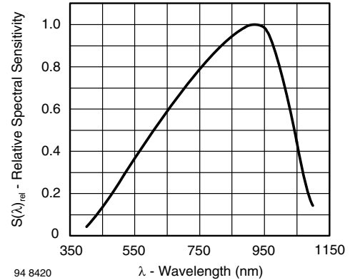
Fig. 6 - Relative Spectral Sensitivity vs. Wavelength
