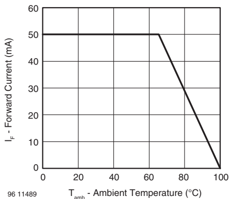
Fig. 1 - Forward Current vs. Ambient Temperature for AllnGaP
