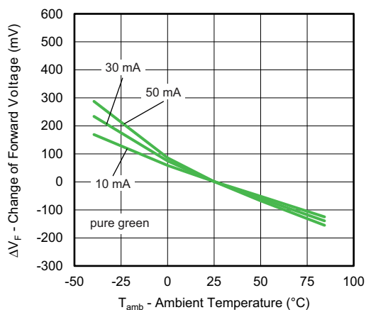
Fig. 15 - Change of Forward Voltage vs. Ambient Temperature
