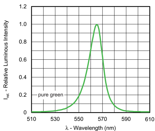
Fig. 10 - Relative Intensity vs. Wavelength
