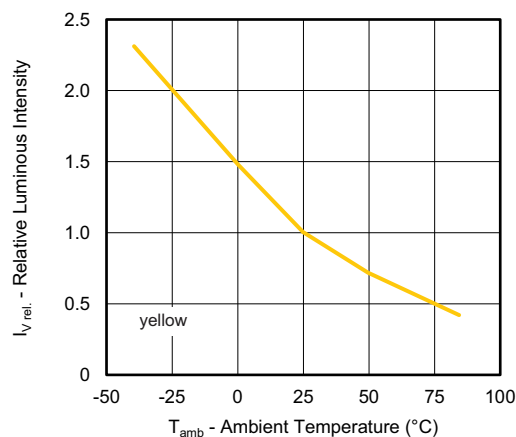
Fig. 7 - Relative Luminous Intensity vs. Ambient Temperature
