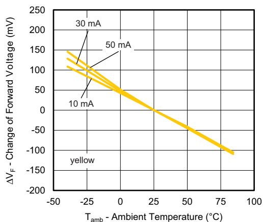
Fig. 9 - Change of Forward Voltage vs. Ambient Temperature
