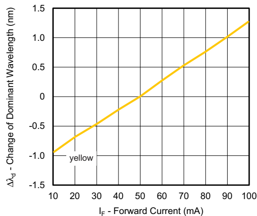
Fig. 6 - Change of Dominant Wavelength vs. Forward Current
