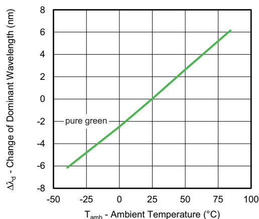
Fig. 14 - Change of Dominant Wavelength vs. Ambient Temperature
