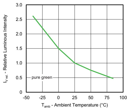
Fig. 13 - Relative Luminous Intensity vs. Ambient Temperature
