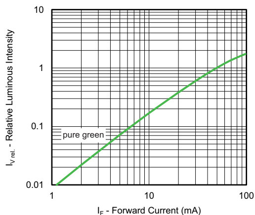
Fig. 11 - Relative Luminous Intensity vs. Forward Current
