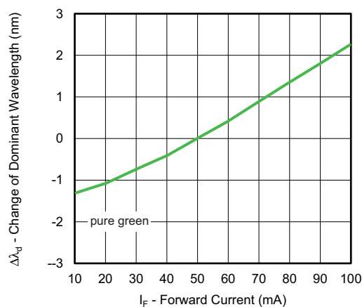
Fig. 12 - Change of Dominant Wavelength vs. Forward Current
