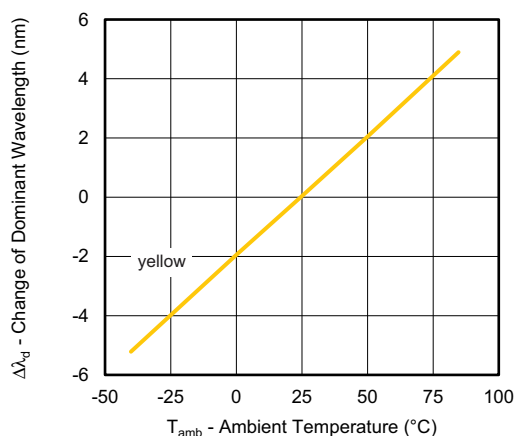
Fig. 8 - Change of Dominant Wavelength vs. Ambient Temperature
