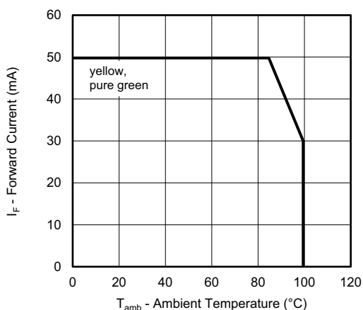
Fig. 1 - Maximum Permissible Forward Current vs. Ambient Temperature
