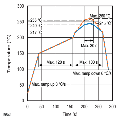
Fig. 9 - Lead (Pb)-free Reflow Solder Profile acc. J-STD-020
