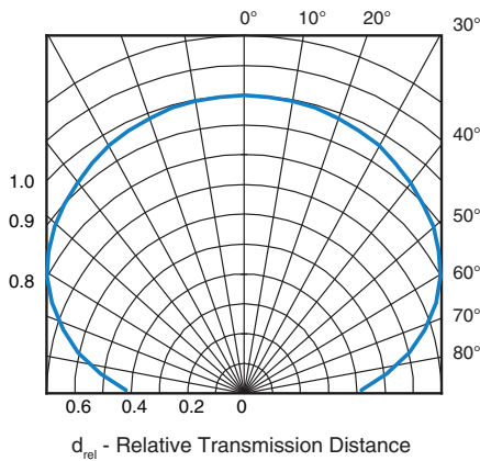
Fig. 11 - Horizontal Directivity
