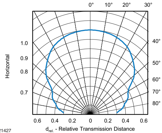
Fig. 11 - Horizontal Directivity
