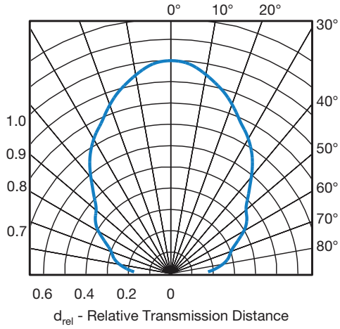
Fig. 11 - Horizontal Directivity
