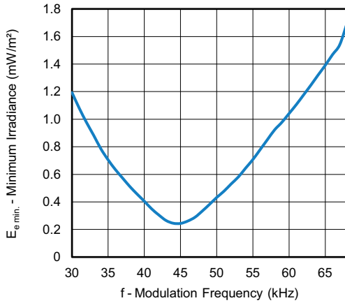
Fig. 5 - Minimum Irradiance vs. Modulation Frequency
