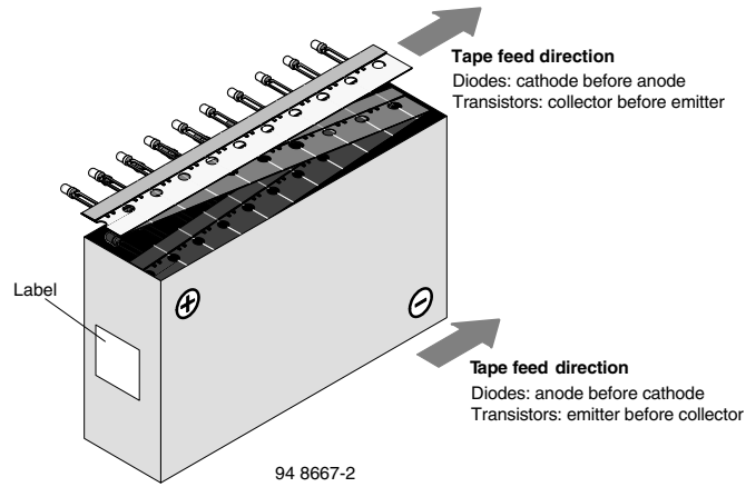
Fig. 24 - Tape Direction
