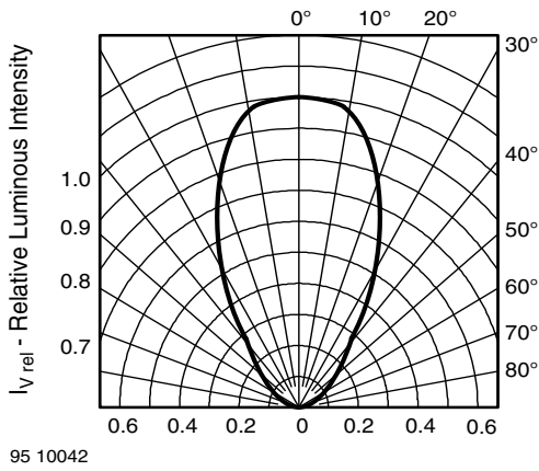
Fig. 4 - Relative Luminous Intensity vs. Angular Displacement
