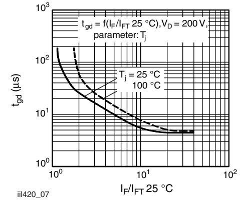
Fig. 7 - Typical Trigger Delay Time
