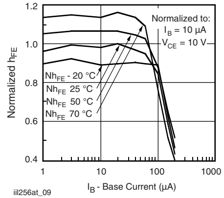
Fig. 9 - Normalized h_{FE} vs. Base Current and Temperature
