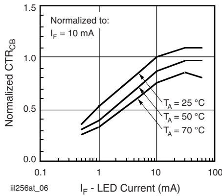
Fig. 6 - Normalized CTR_{CB}
