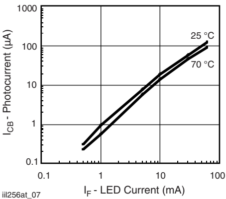
Fig. 7 - Photocurrent vs. LED Current
