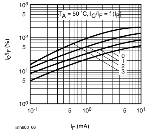
isfh600_06
