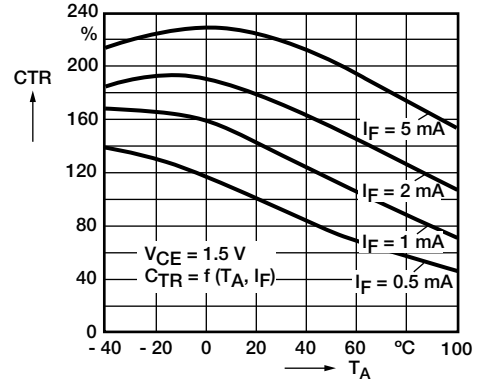
Fig. 4 - Current Transfer Ratio (typ.)
