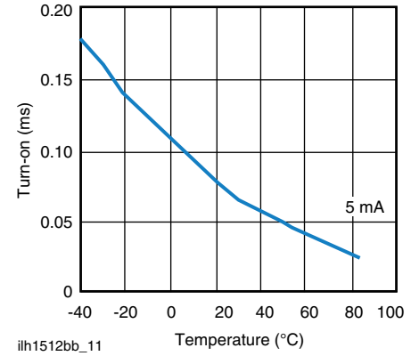
Fig. 11 - Form B Typical Turn-On vs. Temperature
