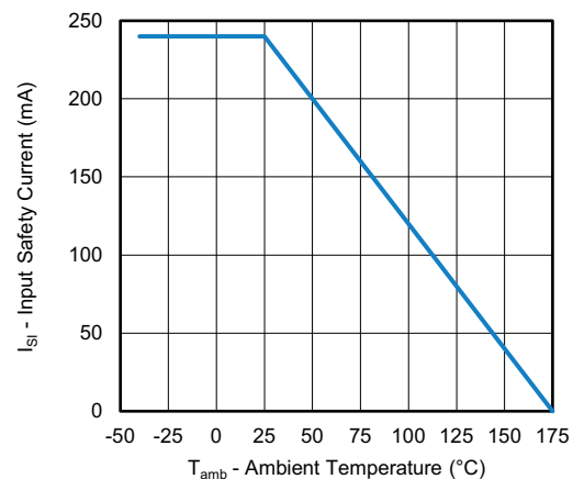
Fig. 3 - Safety Input Current vs. Ambient Temperature
