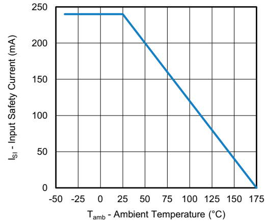
Fig. 4 - Safety Input Current vs. Ambient Temperature
