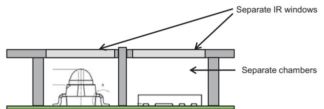
Fig. 12 - Emitter and Detector Totally Separated
