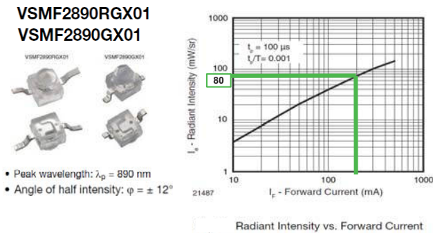
Fig. 9 - VSMF2890GX01 and Radiant Intensity Diagram
