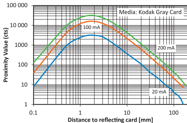
Fig. 1 - Proximity Value vs. Distance
