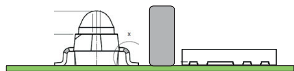
Fig. 7 - Light Barrier in-between IRED and Sensor The emitter package in fig. 7 is called a gullwing package.
