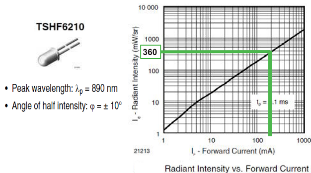
Fig. 10 - TSHF6210 and Radiant Intensity Diagram
