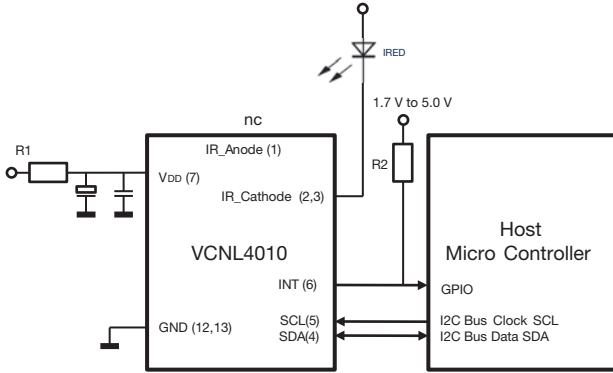
Fig. 3 - VCNL4010 Circuitry with an External IRED
