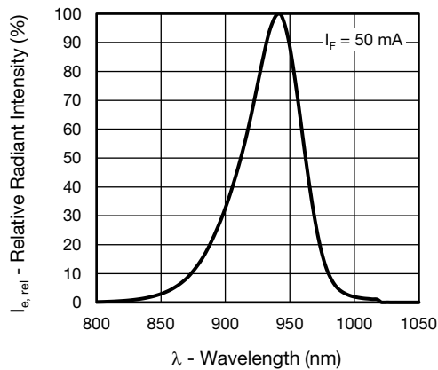
Fig. 1 - Relative Spectral Emission \phi_{e,rel} = f(\lambda)
