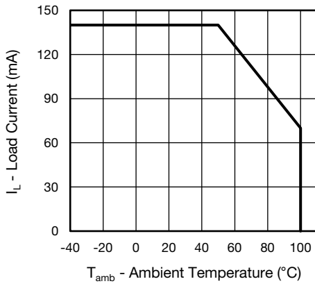
Fig. 4 - Maximum Load Current vs. Ambient Temperature
