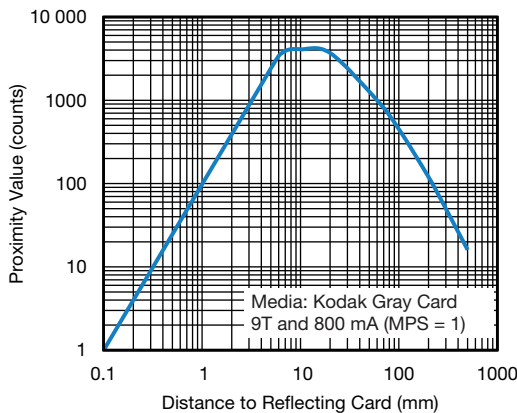
Fig. 16 - Proximity Value vs. Distance for PS_IT= 9T and I_IRED = 800 mA
